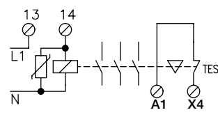
Controlled monitoring of external JOKAB Safety's expansion relays.
