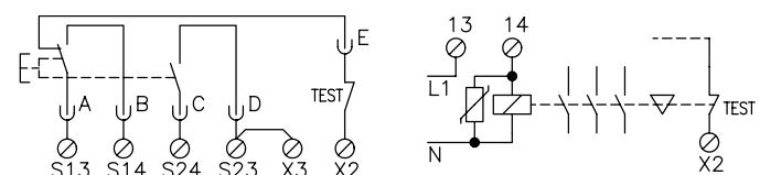
Enabling device, JSHD4. Stop condition is given in both top and bottom PB positions.
