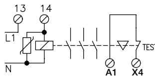
Controlled monitoring of external contactor, relay, valve or ABB Jobab Safety's expansion relays.
